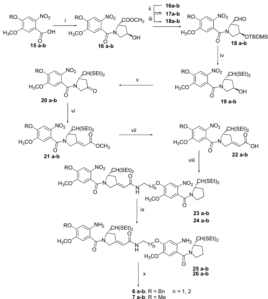
Scheme 2. Reagents and conditions: (i) \text{SOCl}_2 , \text{C}_6\text{H}_6 , trans -4-hydroxy-L-proline methylester hydrochloride, \text{Et}_3\text{N} , \text{H}_2\text{O} , THF, 0^\circ\text{C} , 1 h, 75–80%; (ii) TBDMS-Cl, \text{CH}_2\text{Cl}_2 , 12 h, rt, 90–92%; (iii) DIBAL-H, \text{CH}_2\text{Cl}_2 , -78^\circ\text{C} , 45 min, 65–68%; (iv) EtSH, TMS-Cl, \text{CHCl}_3 , 18 h, rt, 72–75%; (v) TPAP-NMO, \text{CH}_2\text{Cl}_2 -MeCN, 2.5 h, rt, 76–78%; (vi) methyl diethylphosphonoacetate, NaH, THF, 0^\circ\text{C} , 2 h, 80–84%; (vii) 1 N LiOH, THF- \text{H}_2\text{O} -MeOH, 2 h, rt, 83–87%; (viii) EDCl-HOBt, compound 14a-b , \text{CH}_2\text{Cl}_2 - \text{H}_2\text{O} , 24 h, rt, 54–60%; (ix) \text{SnCl}_2 - 2\text{H}_2\text{O} , MeOH, reflux, 3 h, 70–75%; (x) \text{HgCl}_2 - \text{CaCO}_3 , \text{CH}_3\text{CN} - \text{H}_2\text{O} , 12 h, rt, 48–55%.
