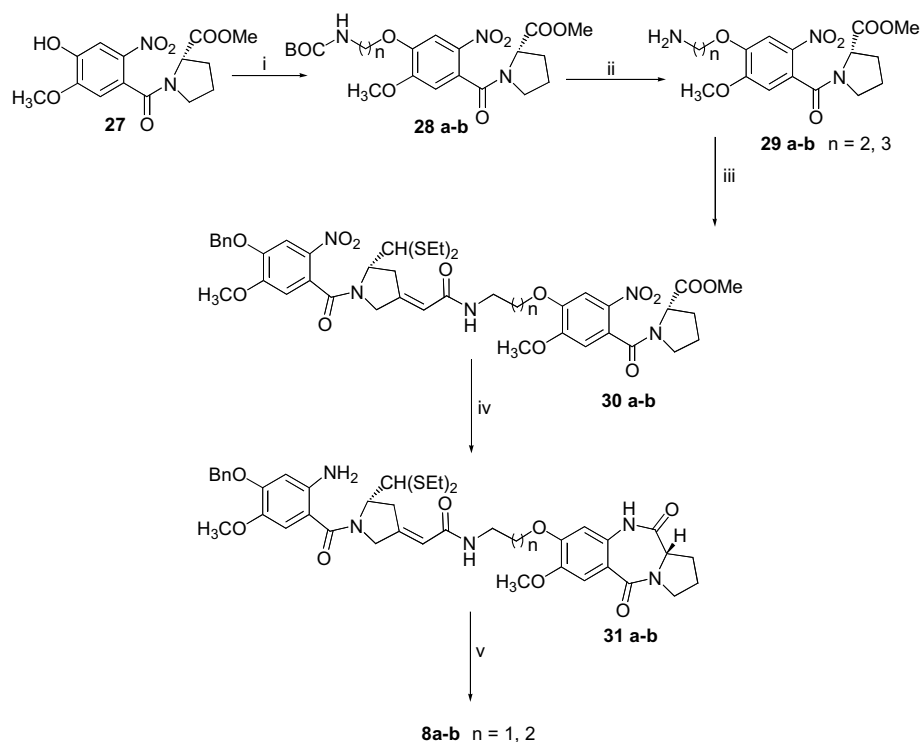
Scheme 3. Reagents and conditions: (i) Boc-protected bromo alkylamine, K_2CO_3 , DMF, rt, 24 h, 80–82%; (ii) TFA, CH_2Cl_2 , 8 h, rt; (iii) EDCI-HOBt, compound 22a , CH_2Cl_2 - H_2O , 24 h, rt, 65–67%; (iv) SnCl_2 \cdot 2H_2O , MeOH, reflux, 3 h, 76–78%; (v) HgCl_2 - CaCO_3 , CH_3CN - H_2O , 12 h, rt, 51–53%.
